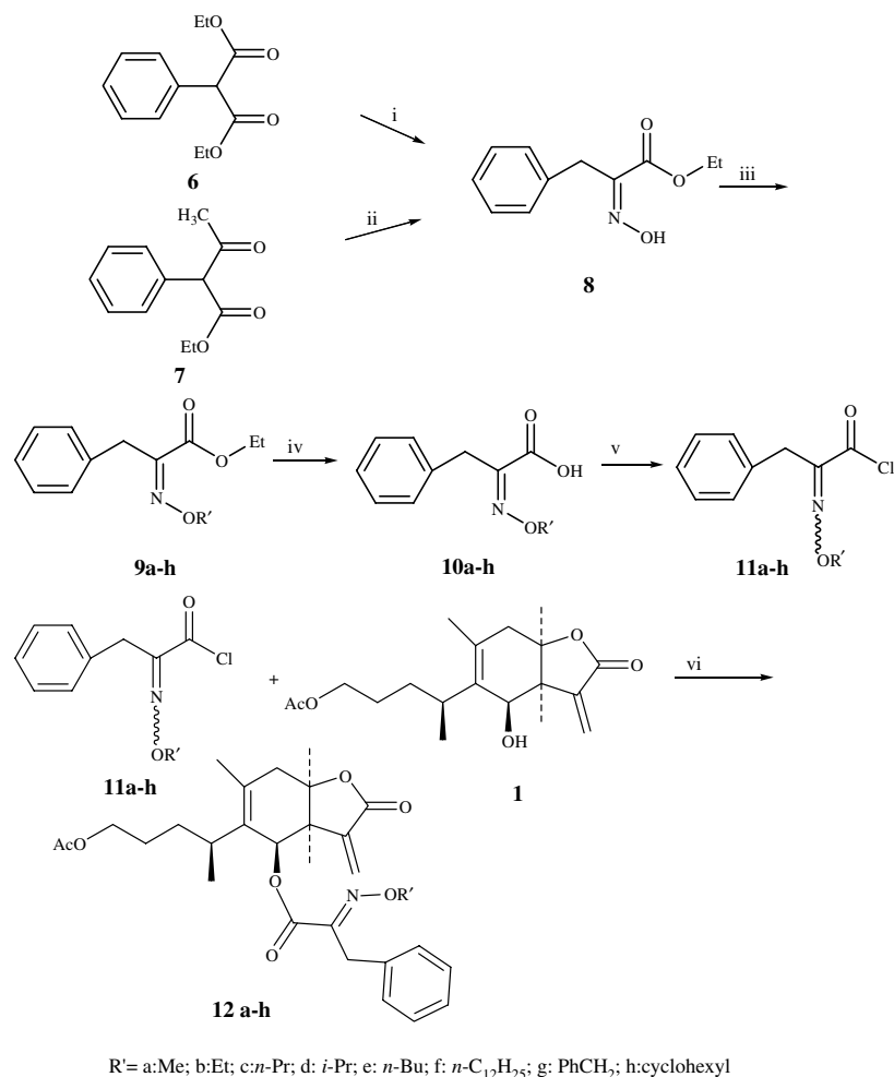
Scheme 1. Reagents and conditions: (i) EtONO/NaOEt, 0 °C; (ii) EtONO/80% H 2 SO 4 , 0–5 °C; (iii) bromoalkane, K 2 CO 3 /acetone, 30–35 °C; (iv) NaOH, H 2 O/EtOH, H 3 O + ; (v) SOCl 2 , CH 2 Cl 2 ; (vi) DMAP/CH 2 Cl 2 .
